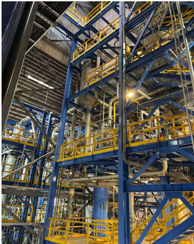
PORT CARTIER RTP™ PLANT: 10 million gpy
